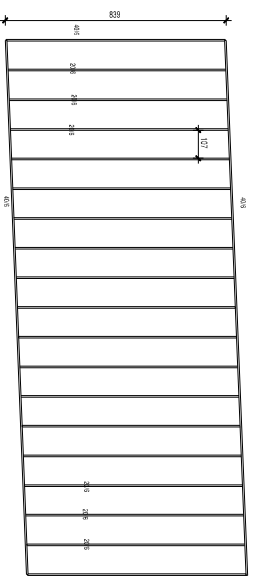
D08 GARDE-CORPS 1/10
