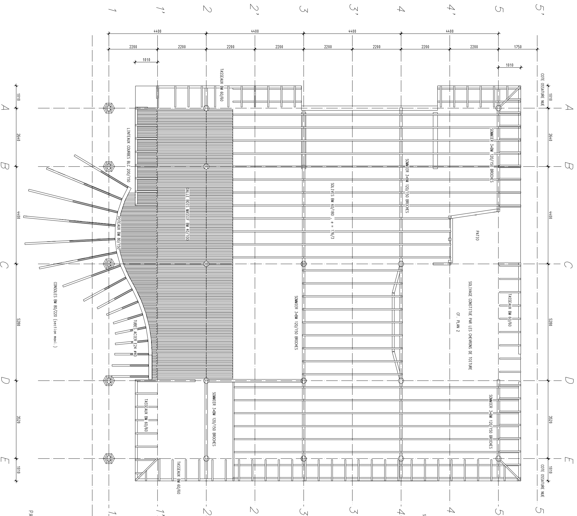
PLAN 1 1/50
